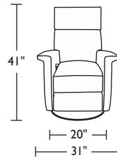
FNL-RV5-ST
